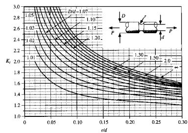
Spotts, Fig. 2-11, Peterson
