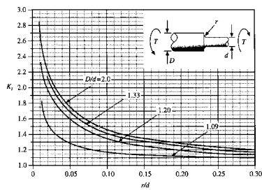
Spotts, Fig. 2-10, Peterson
