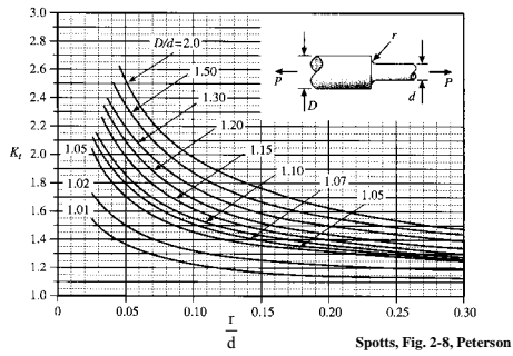
Spotts, Fig. 2-8, Peterson
