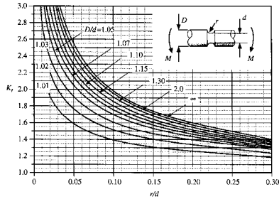
Spotts, Fig. 2-12, Peterson
