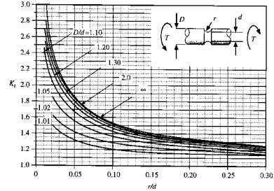
Spotts, Fig. 2-13, Peterson
