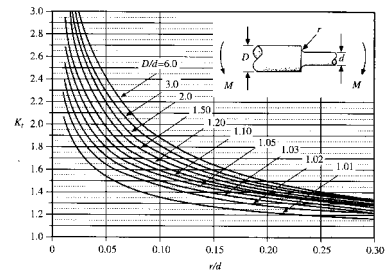
Spotts, Fig. 2-9, Peterson
